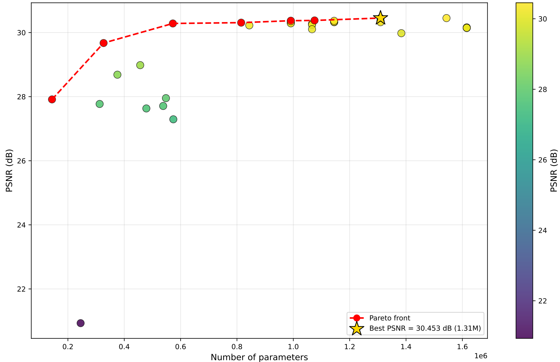
PSNR vs #Parameters — SRFormer
